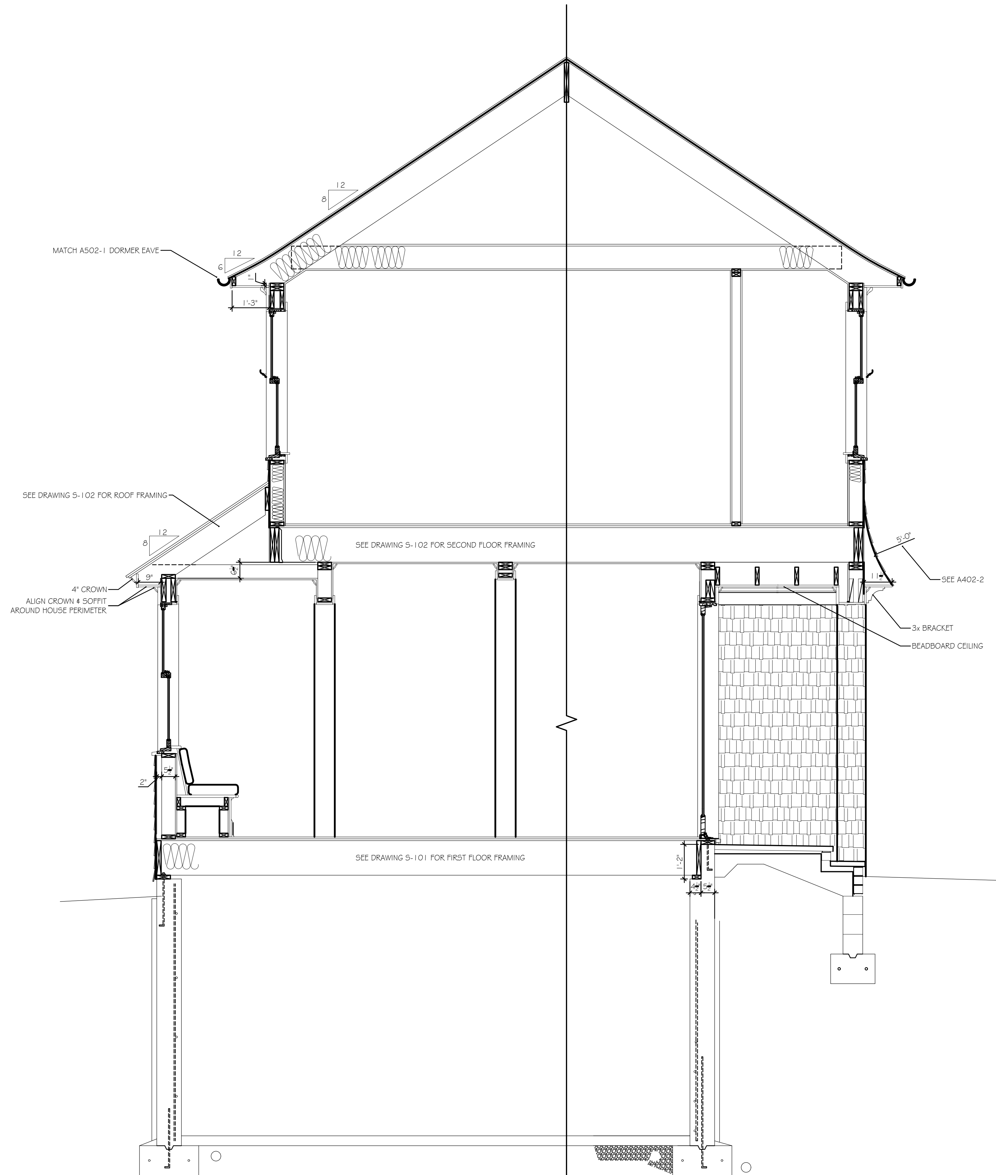
1 SECTION- MUDROOM PORCH/BREAKFAST BAY SCALE: 1/2" = 1'-0" NOTE: MATCH DRAWING A501/1 UNLESS NOTED OTHERWISE
